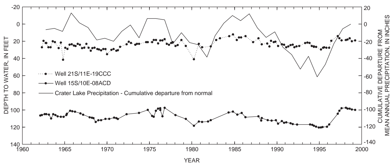
Figure 31. Static water levels in two long-term observation wells in the upper Deschutes Basin, Oregon, and cumulative departure from normal annual precipitation at Crater Lake, Oregon, 1962–98.
