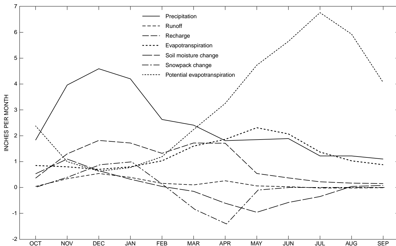
Figure 8. Mean monthly components of the basinwide water budget, estimated using the Deep Percolation Model for water years 1962–97.
