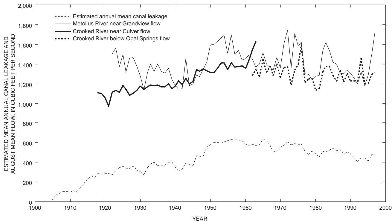
Figure 23. August mean flows of the Crooked River below Opal Springs, the Metolius River near Grandview, and estimated annual mean leakage from irrigation canals, 1905–97.
