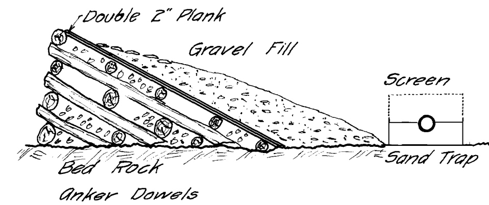
SKETCH LOG CRIB DAM ROCK FILLED
