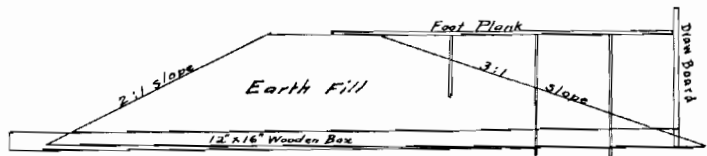
Cross Section of Dam at Outlet. Scale: 1" = 6'.
