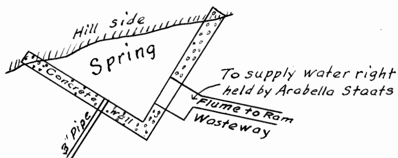
Plan of Proposed Head Works Scale 1" = 10'
