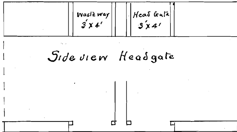
Top view of Headgate.
