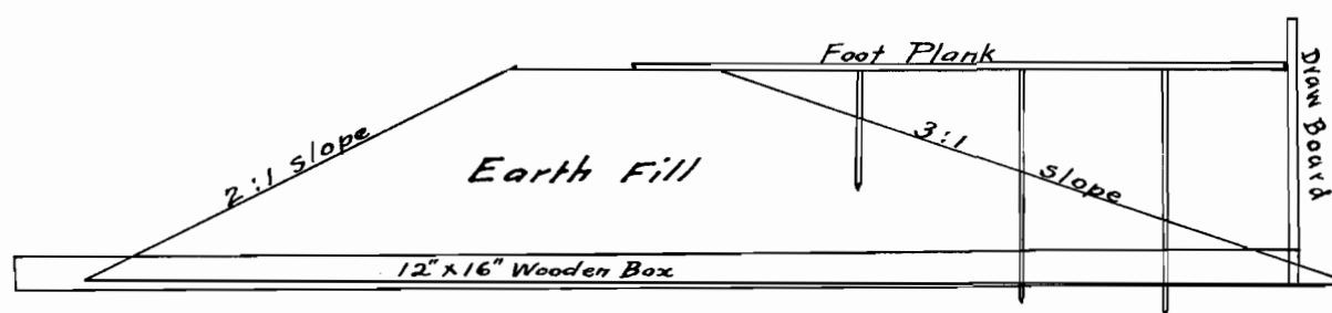
Cross Section of Dam at Outlet. Scale: 1" = 6'
