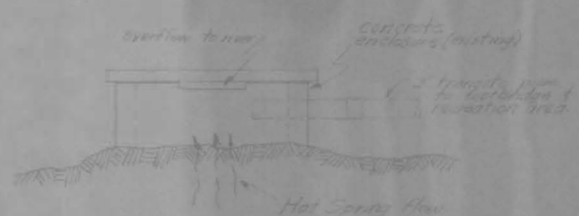
HOT SPRING HEADWORKS Scale 1/2"=1'-0"
