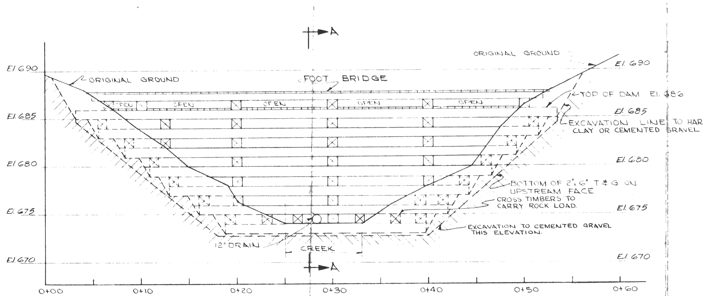
PROFILE OF DAM AXIS SCALE: 1" = 5'
