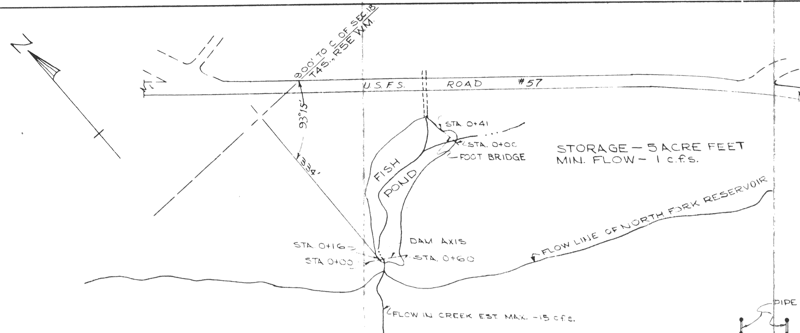
LOCATION PLAN SCALE: 1" = 100'
