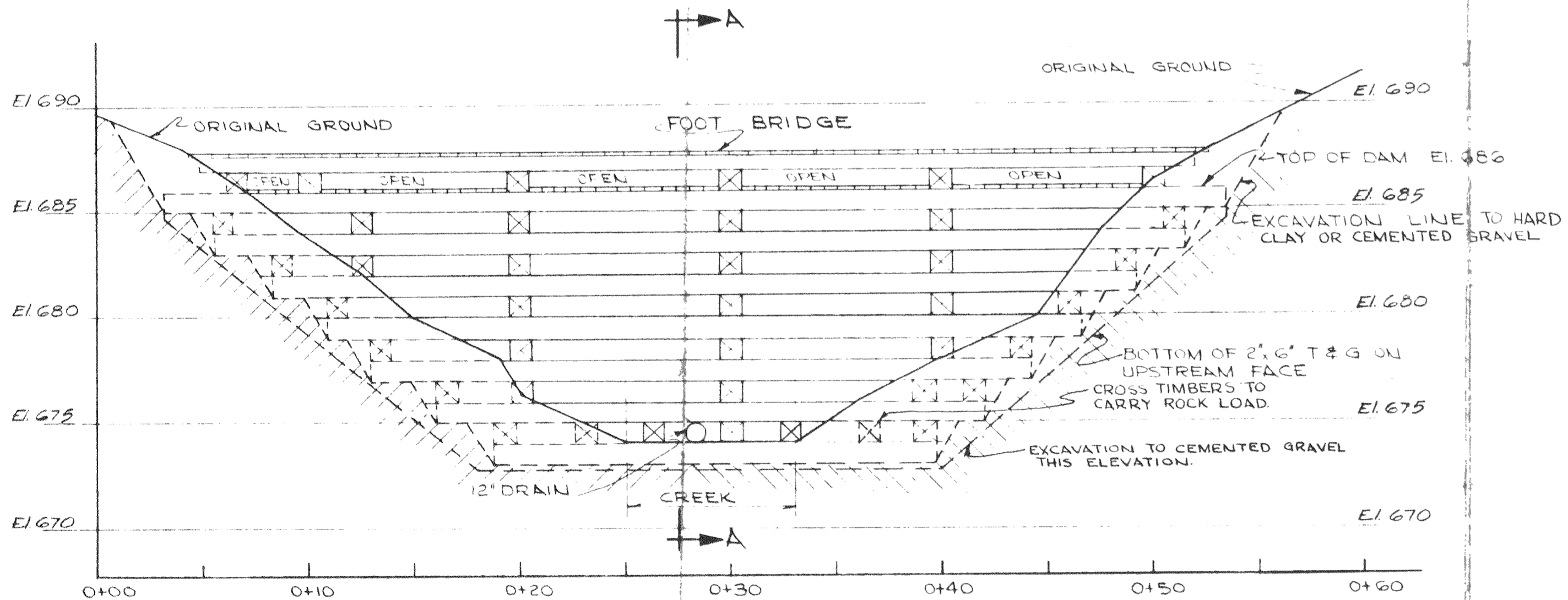
PROFILE OF DAM AXIS SCALE: 1" = 5'
