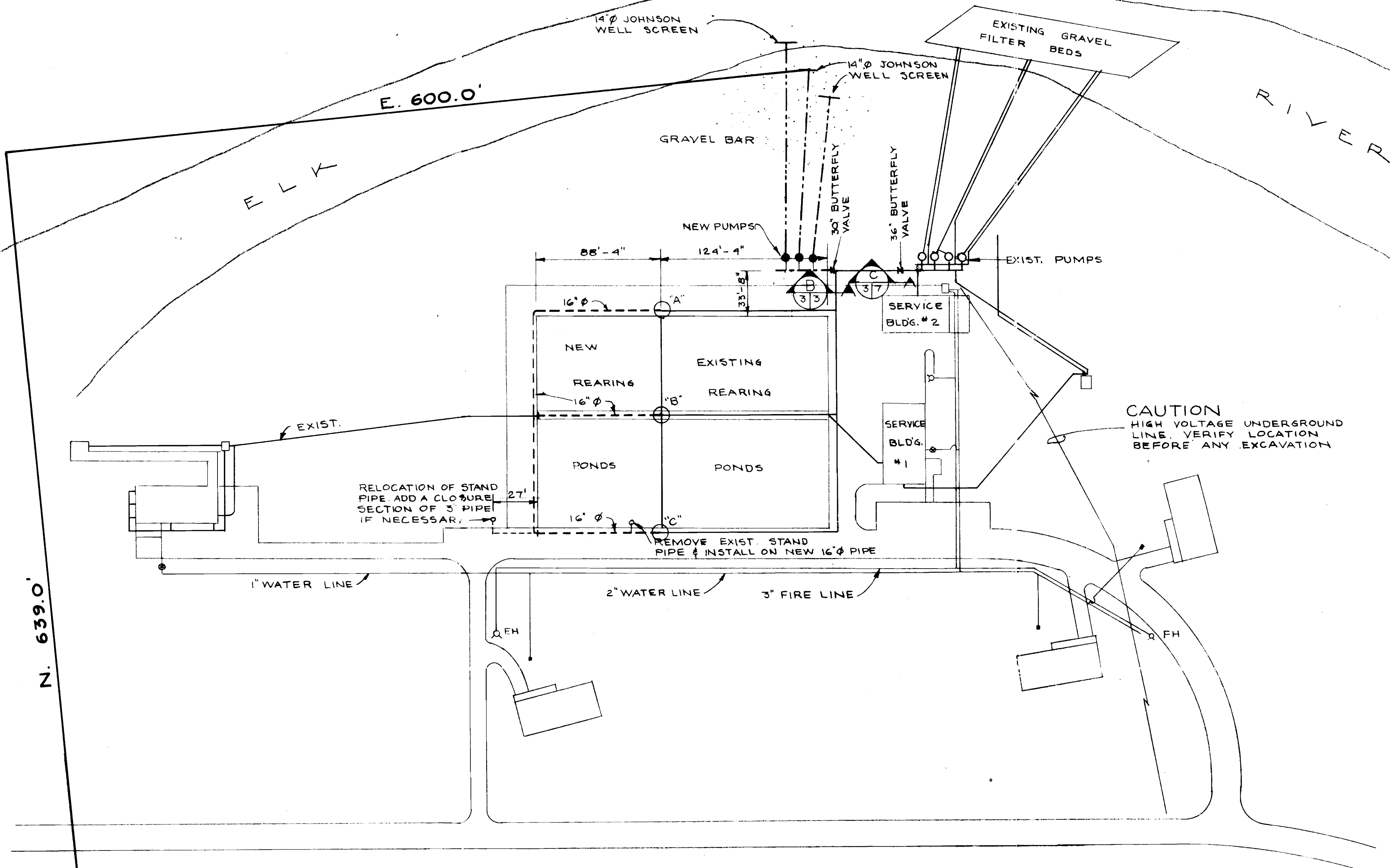
PLUMBING PLAN SCALE: 1" = 50'
