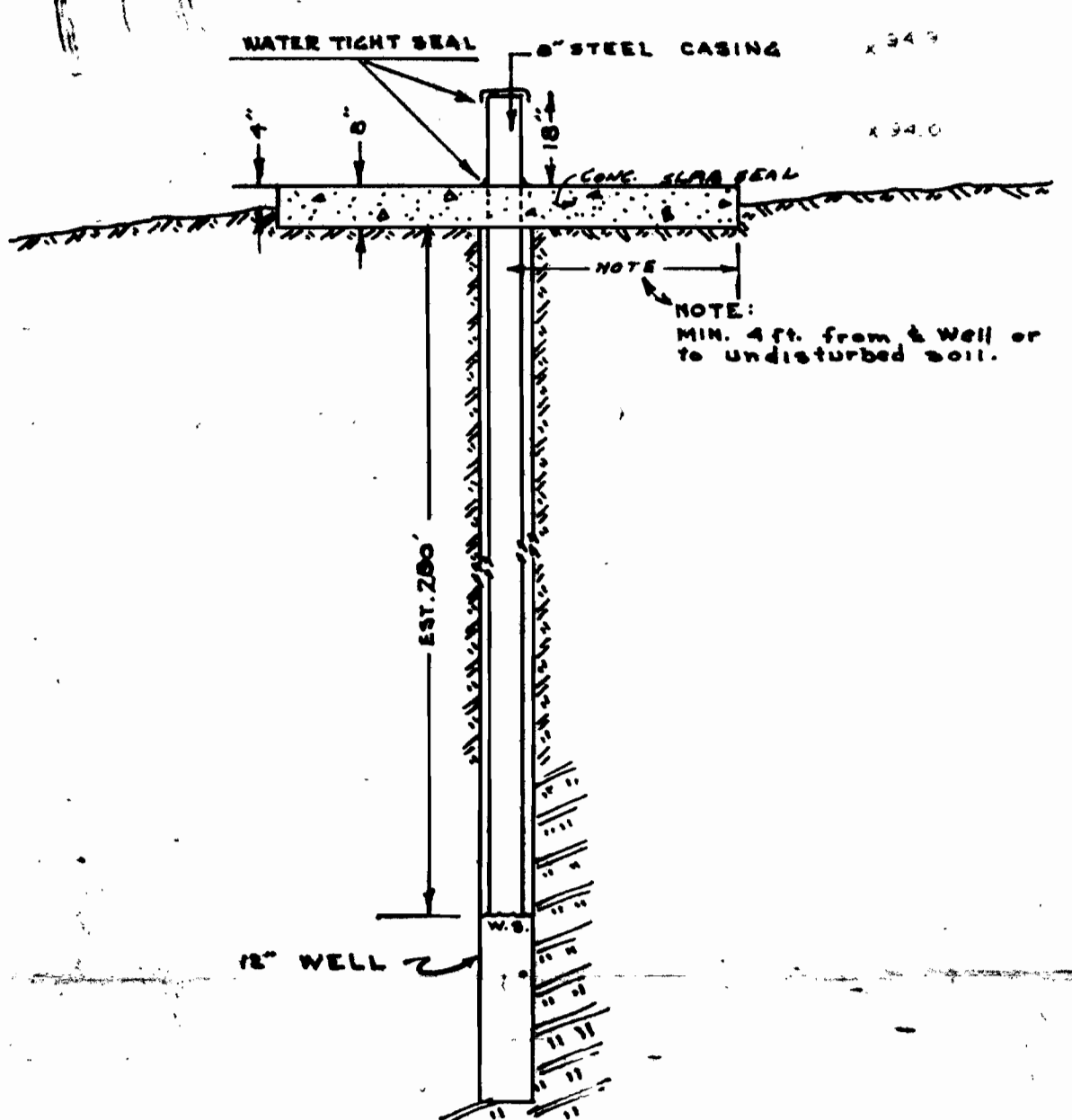
SECTION THRU WELL SCALE 1" = 3'-0"
