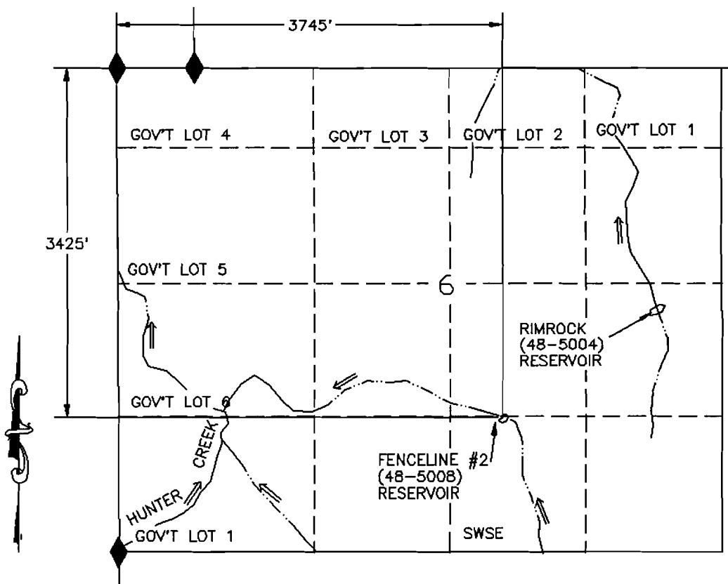
FENCELINE #2 (48-5008) RESERVOIR
