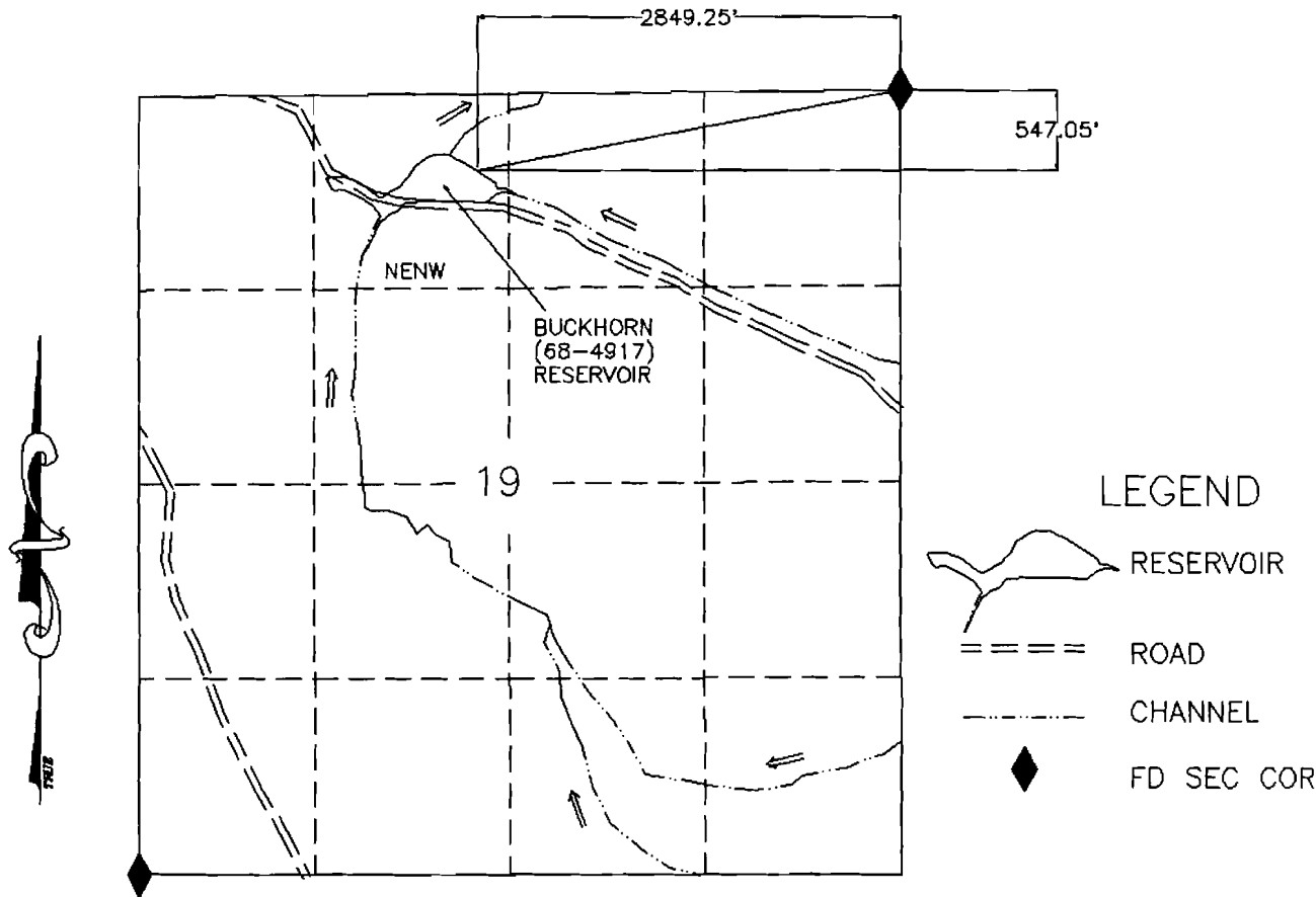
BUCKHORN (68-4917) RESERVOIR
