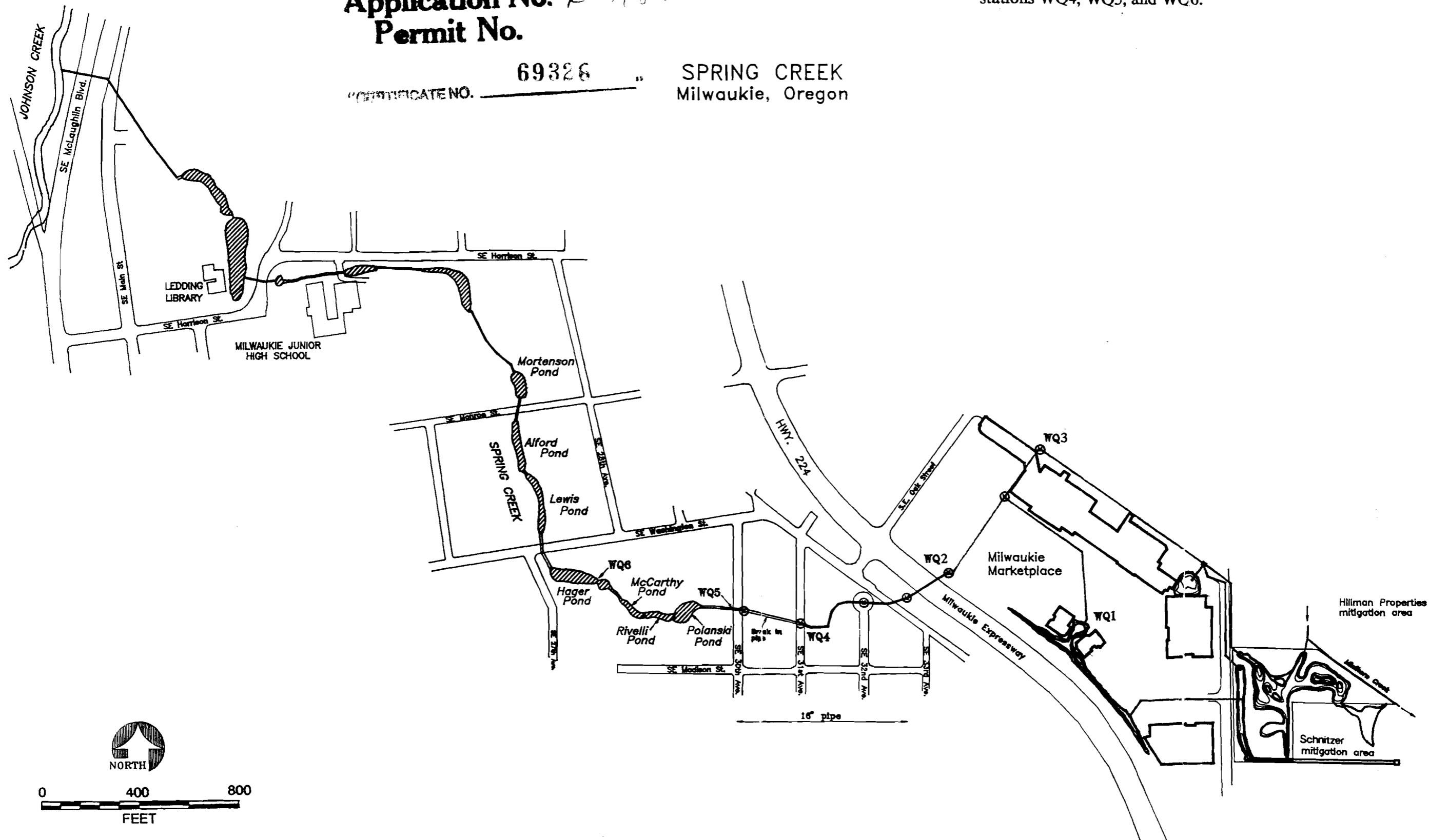
Figure 2. The location of the Milwaukie Marketplace and Spring Creek as it flows to the north into Johnson Creek. Also shown are water quality stations WQ4, WQ5, and WQ6.
