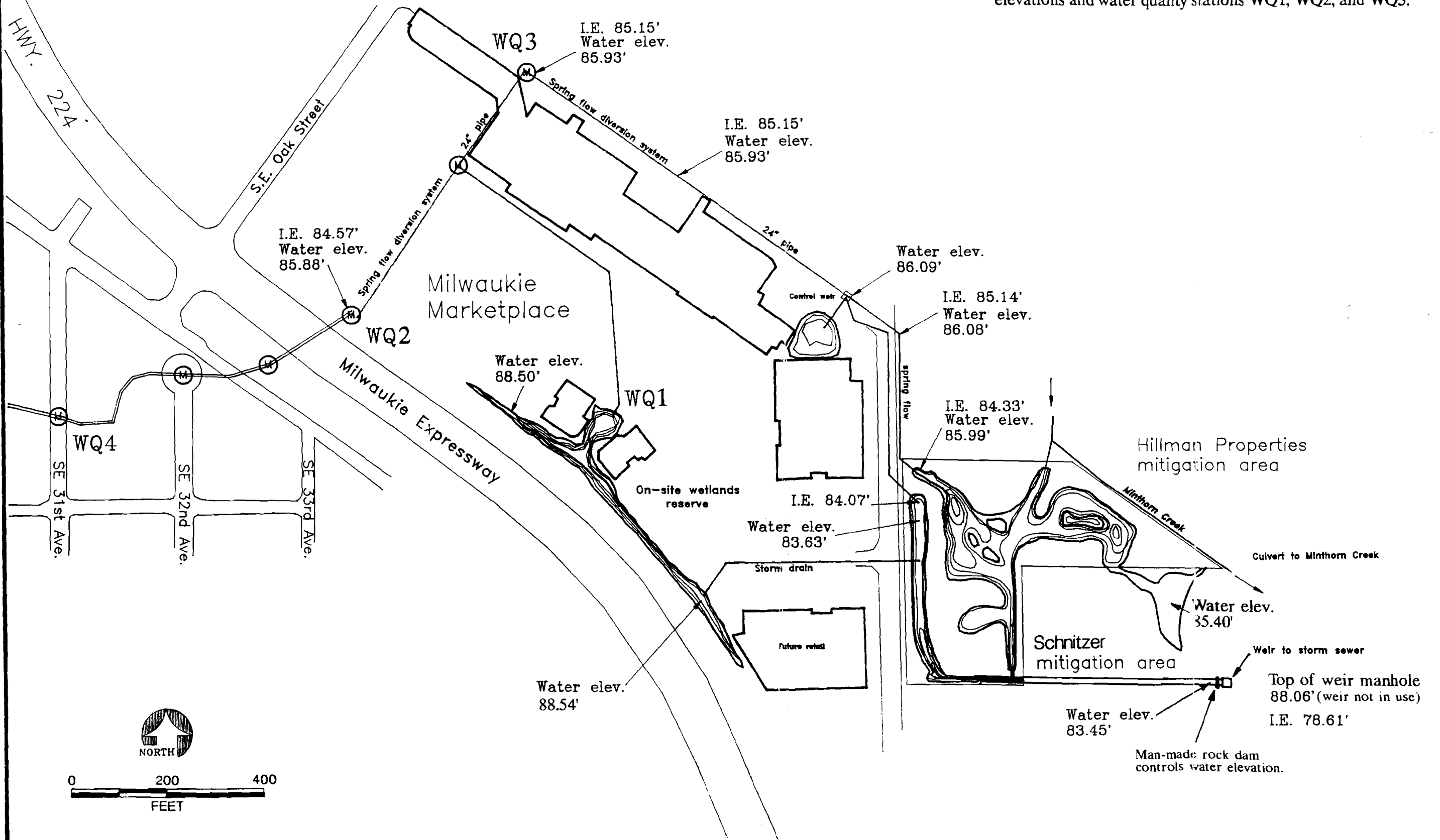
Figure 3. The diversion system beneath the Milwaukie Marketplace showing elevations and water quality stations WQ1, WQ2, and WQ3.
