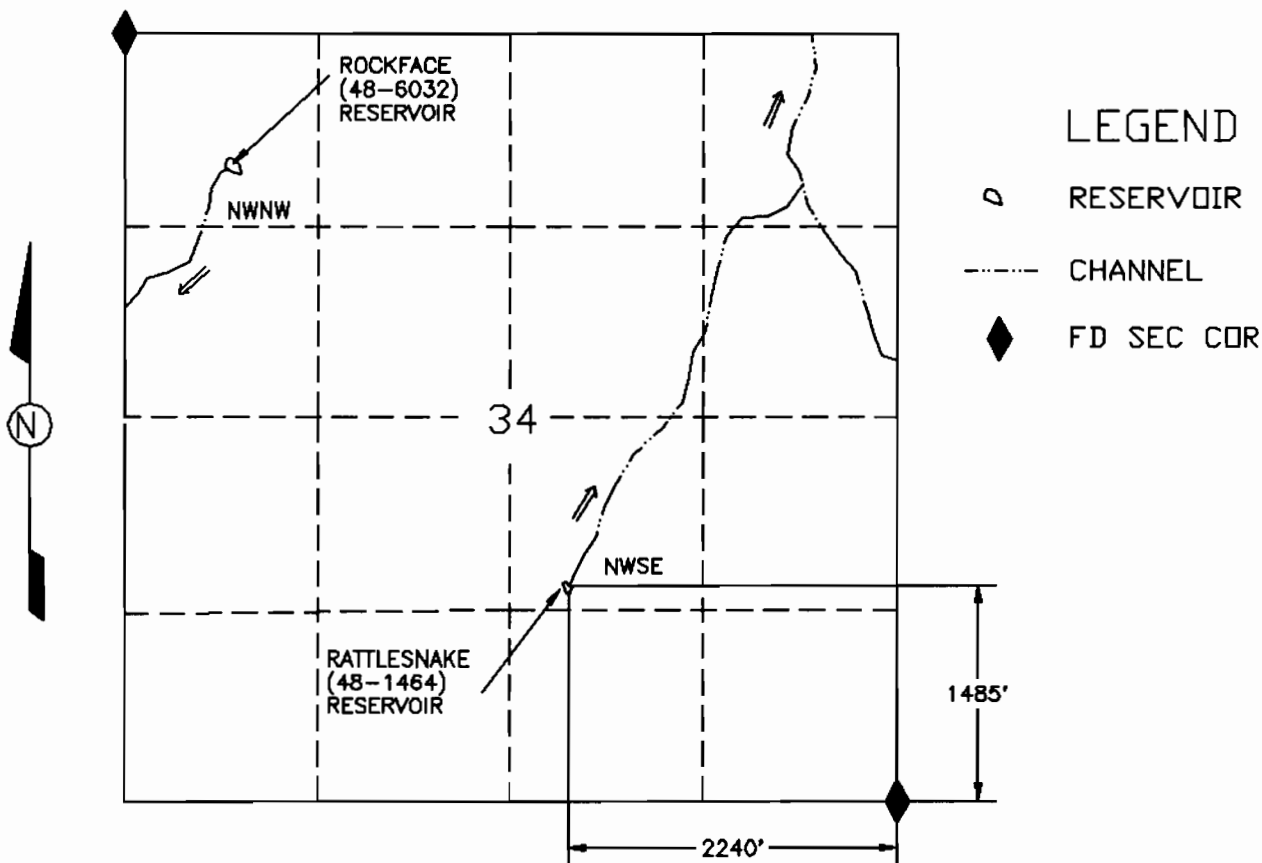
RATTLESNAKE (48-1464) RESERVOIR
