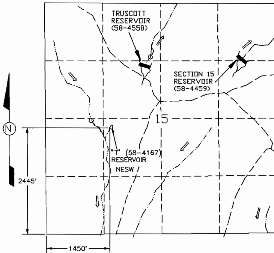
"T" (58-4167) RESERVOIR
