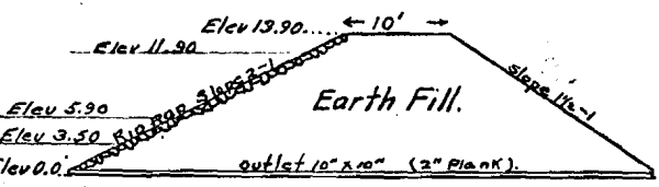
End View Scale 1" = 20'
