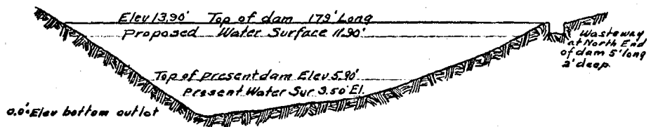
Up Stream View. Scale: Hor 1" = 50' Vert 1" = 20'
