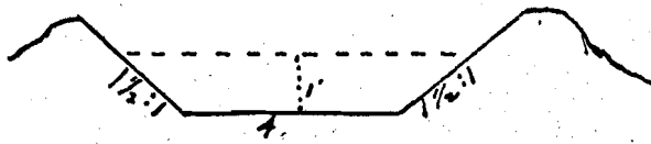
Cross section Canal.
