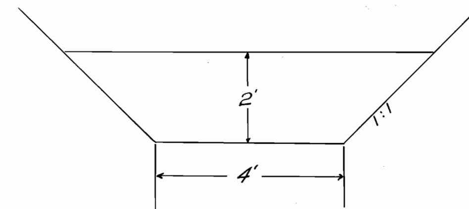
Cross section of Colt Ditch
