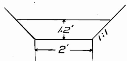
Crosssection of Burkhead Dearinger Ditch
