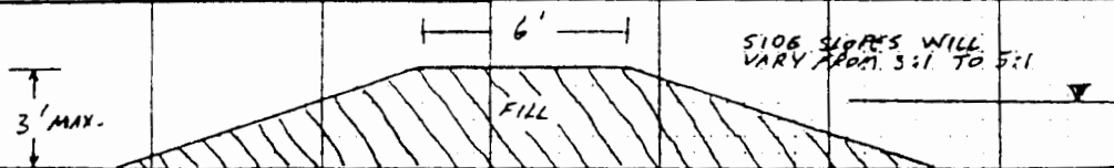
TYPICAL CROSS-SECTION DIKE 1 INCH = 5 FEET
