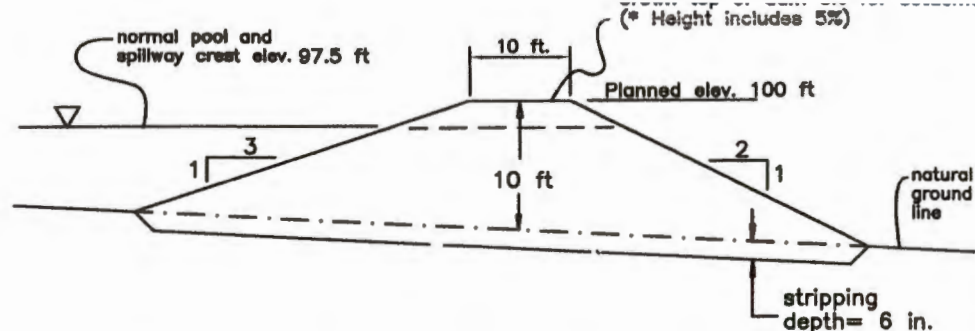
MAXIMUM CROSS SECTION OF DAM
