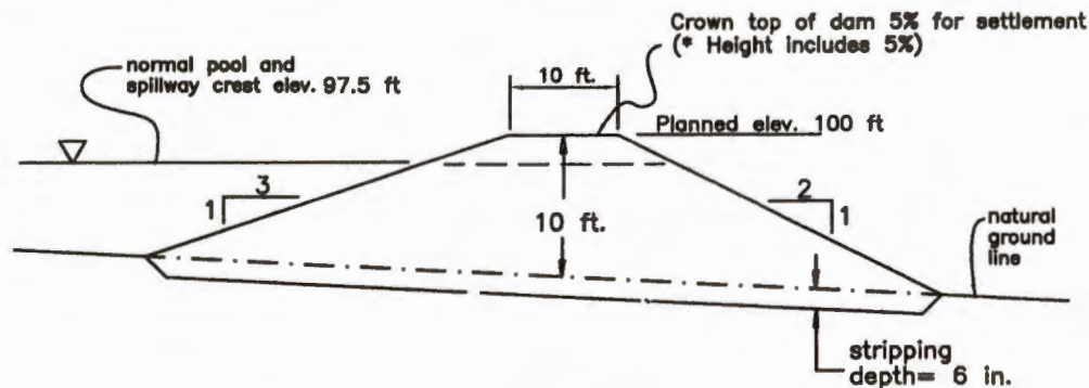
MAXIMUM CROSS SECTION OF DAM
