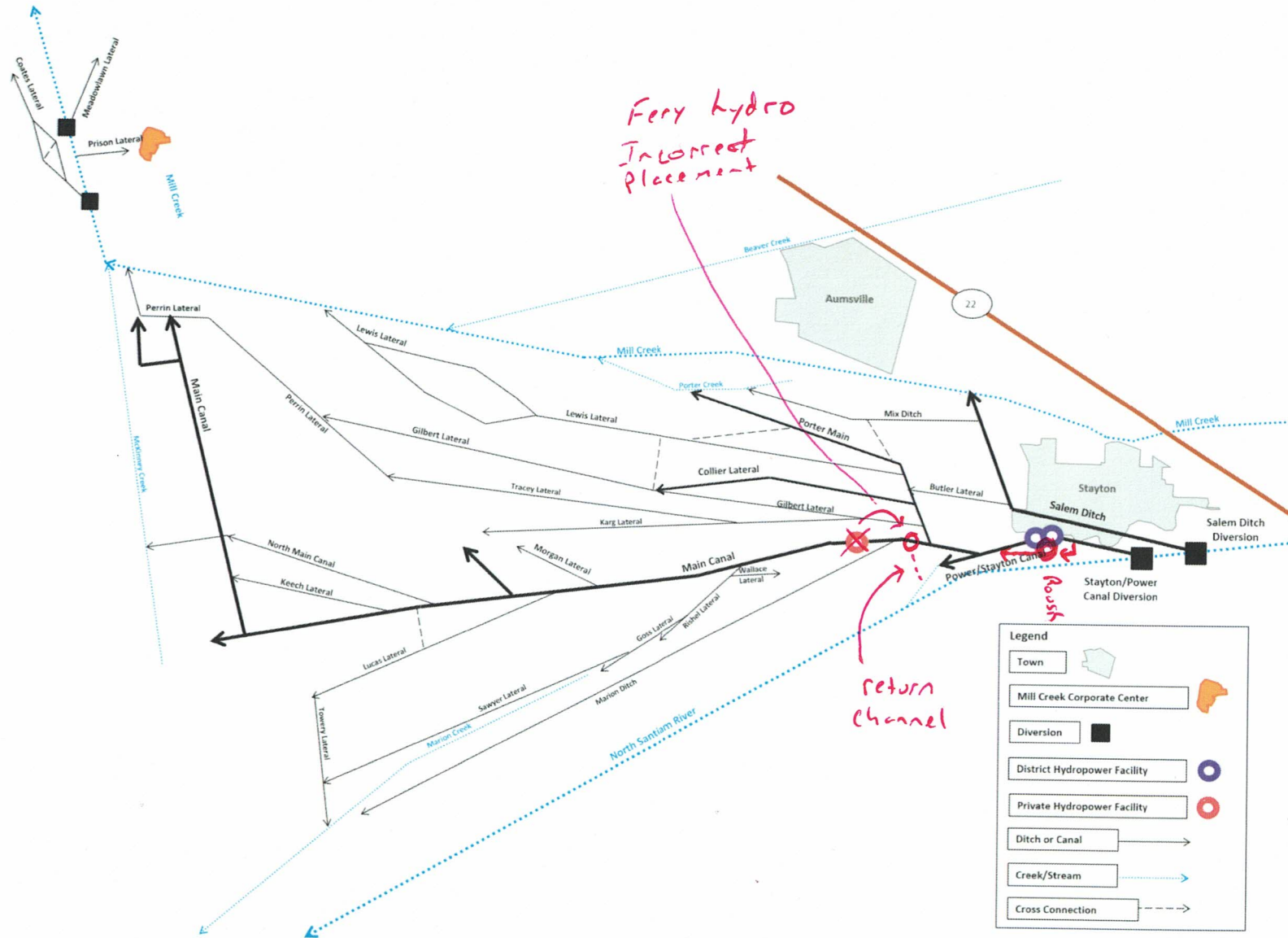
Figure 2-2. Schematic of Santiam Water Control District's Existing Delivery System.
