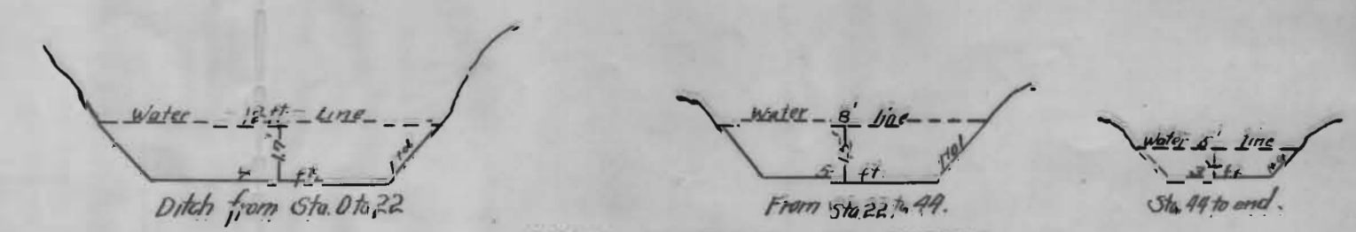
GROSS SECTIONS OF DITCH Scale 5 ft. to 1 in. Grade 0.2% per 100'
