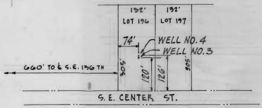
PLOT PLAN - WELLS #3 & #4 1" = 200'
