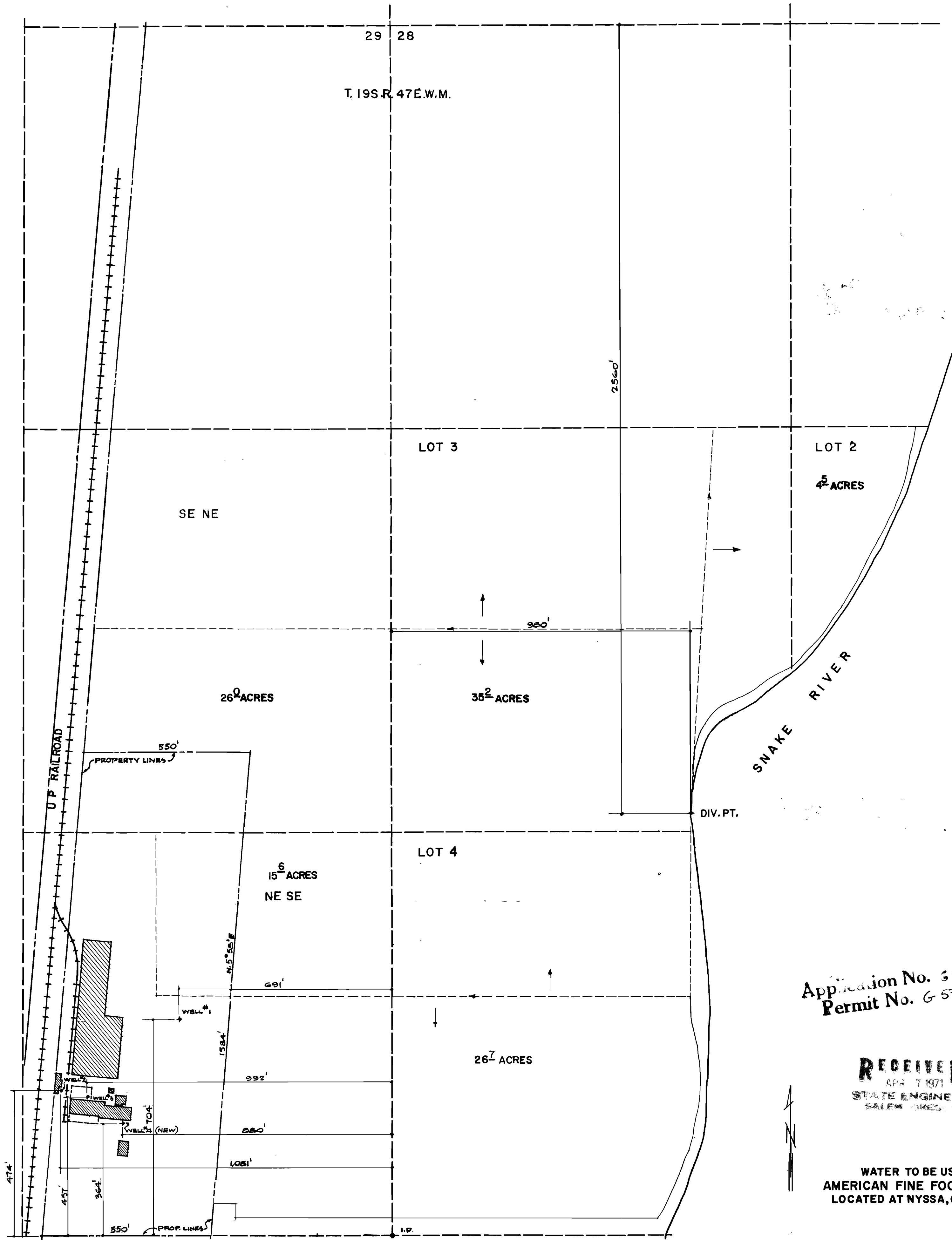
SITE PLAN SCALE = 1" = 200'-0"
