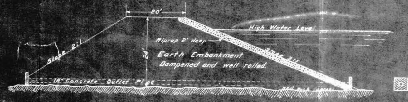
CROSS SECTION OF DAM Scale: 1" = 20'
