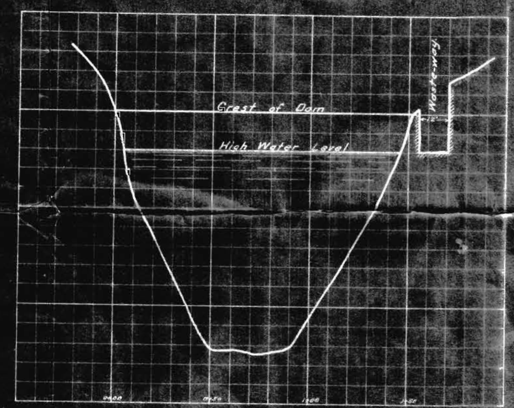
PROFILE OF DAM Scale: Horizontal 1" = 50' Vertical 1" = 10'
