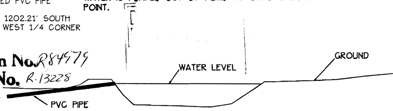
TYPICAL CROSS SECTION OF ALL SEVEN PONDS NO SCALE
