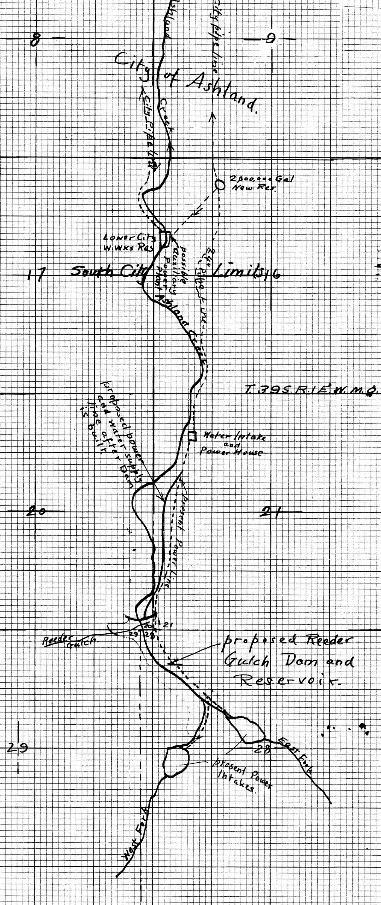
Plat showing General Location from Ashland to proposed Reeder Gulch Reservoir, showing present and proposed arrangement of pipe lines for Water Supply and Power Uses May 1921
