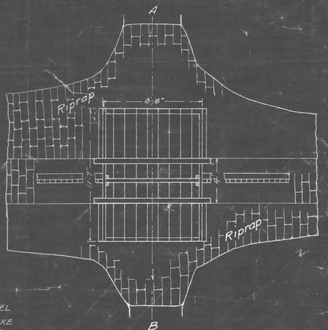
PLAN OF WASTEWAY
