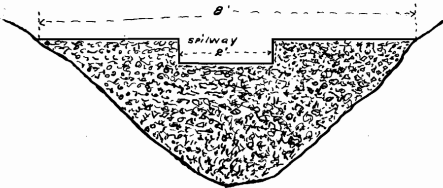
Cross Section of Lower face of concrete dam Scale 1" = 2'
