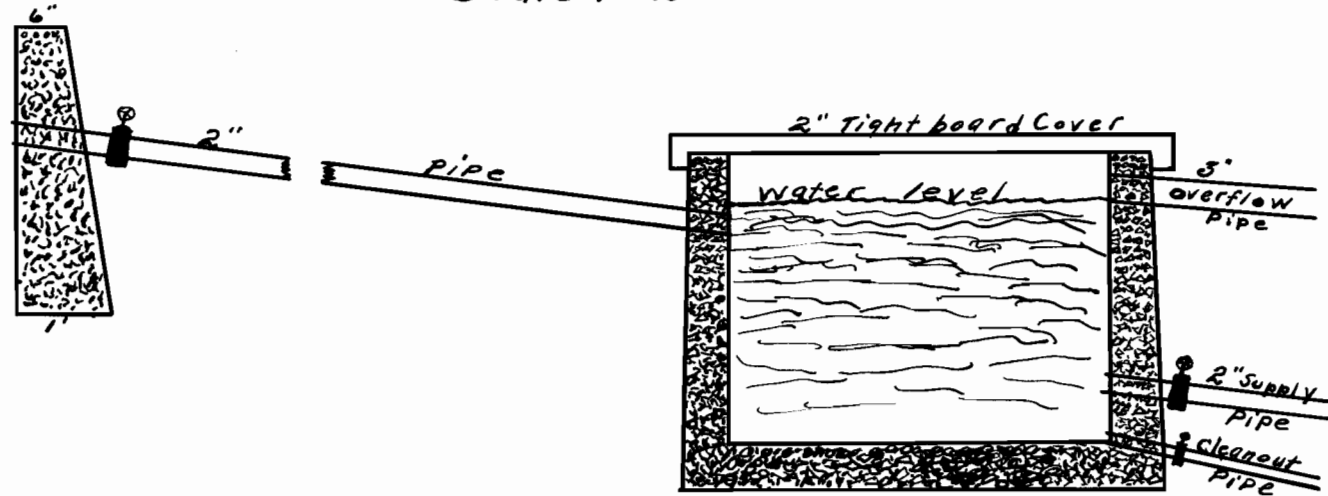
Cross Section of dam and Collecting Reservoir 3'x3'x4' inside Scale 1" = 2'
