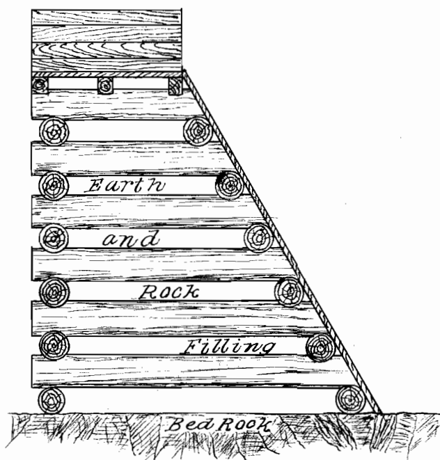
CROSS SECTION OF DAM Scale 1" = 10'
