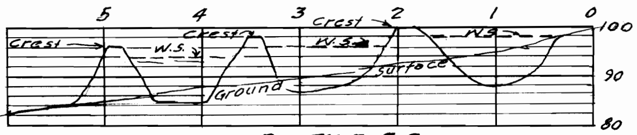
PROFILE A-A Scale: Hor. 100'=1" Vert. 20'=1"
