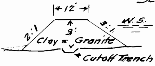
SECTION Scale 20'=1"
