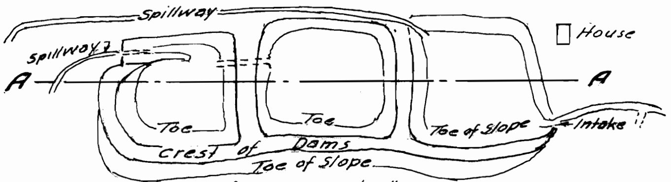
PLAN: Scale 100'=1"
