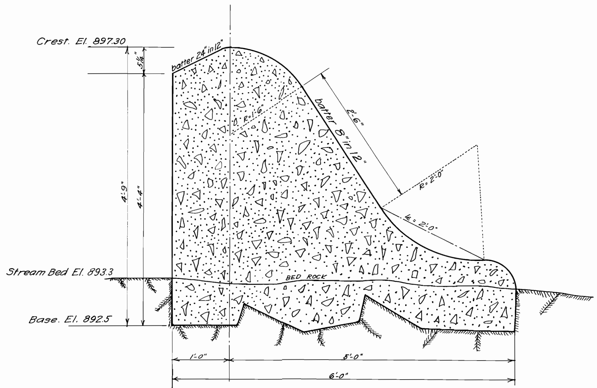
PROFILE OF DAM- SPILLWAY SECTION Scale: 1"=1'
