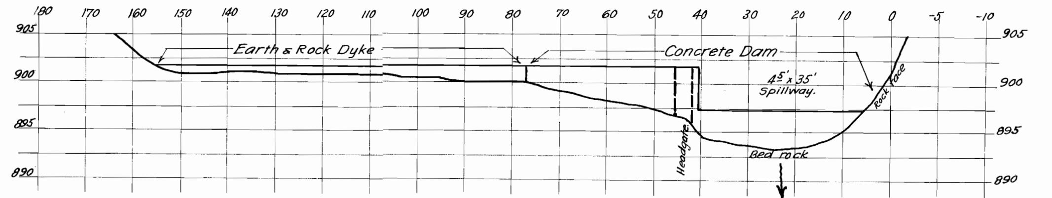
CROSS-SECTION OF DAMSITE Scales: Hor. 1"=20', Vert. 1"=10'
