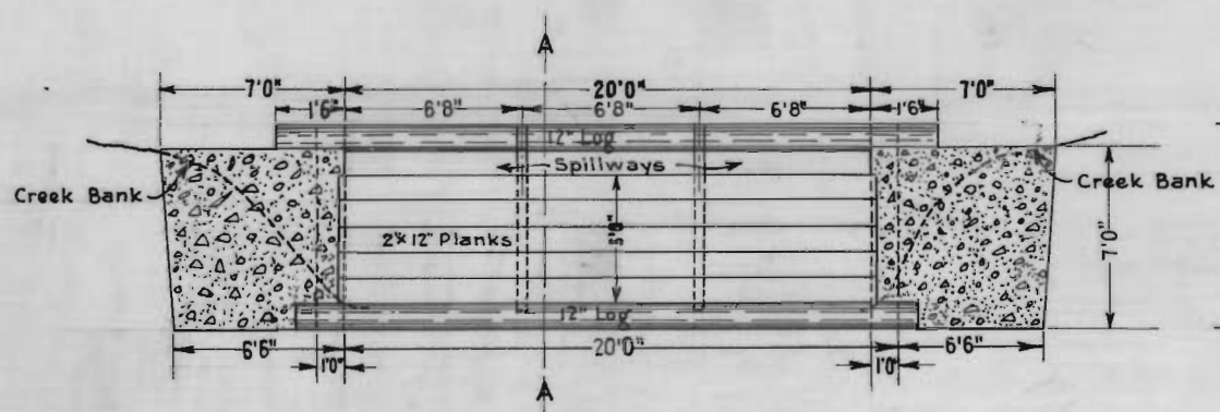
ELEVATION OF DAM Up-stream Side
