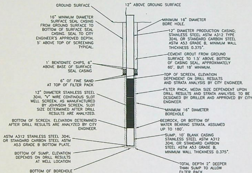
1 TYPICAL ALLUVIAL WATER WELL SCALE: N.T.S.
