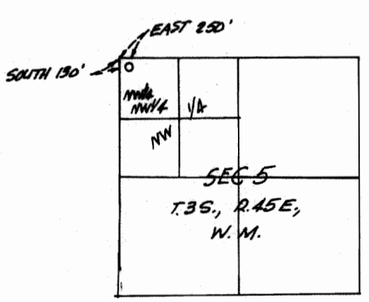
DETAIL POINT OF DIVERSION SCALE 1"=3000'
