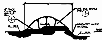
1. SPILLWAY SECTION NTS
