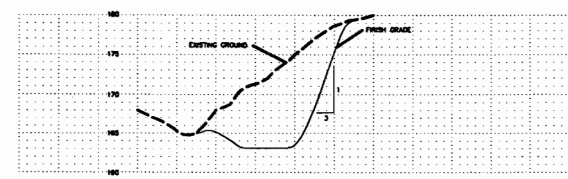
A SECTION C-1 NTS
