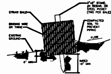
2. EROSION CONTROL - STRAW BALE NTS
