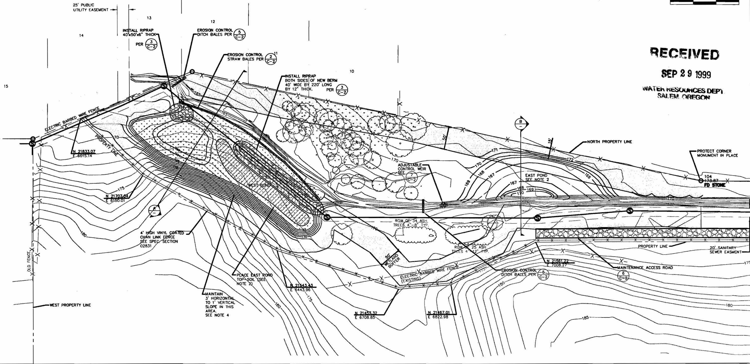
Figure 1 CONSTRUCTION LAYOUT OF THE JONES FARM EAST AND WEST RESERVOIRS
