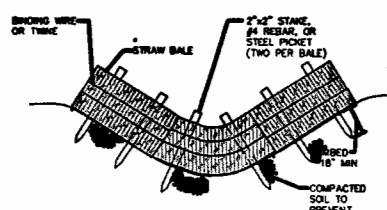
5. EROSION CONTROL - DITCH BALES NTS
