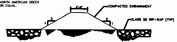
SECTION B
