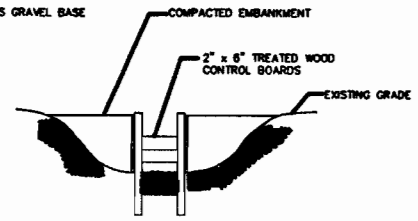
SECTION C
