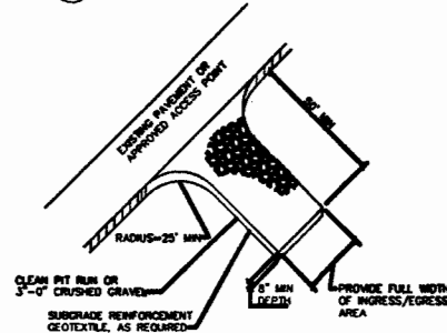
4. GRAVEL CONSTRUCTION ENTRANCE NTS
