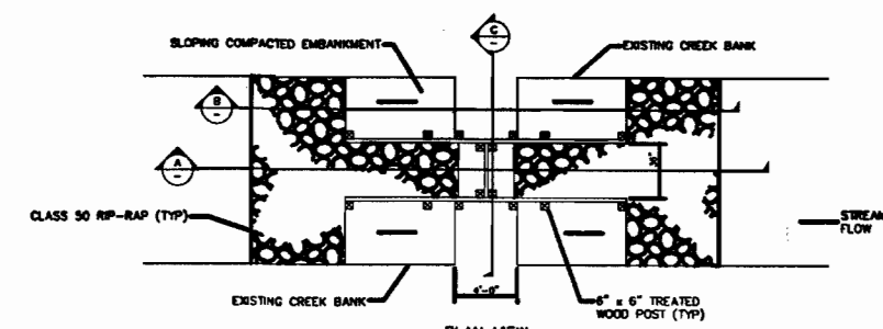
PLAN VIEW
