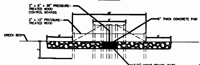
SECTION A
