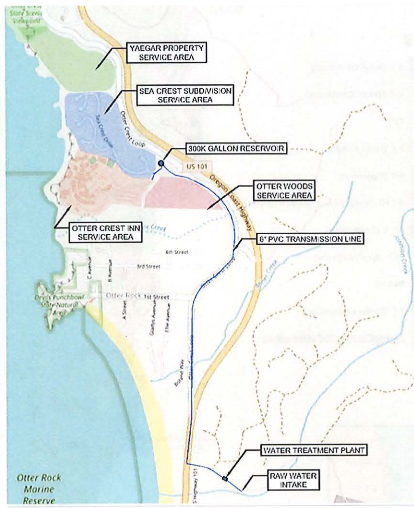
Figure 1 – Water Service Area
