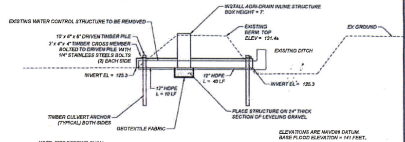
A AGRI-DRAIN SECTION NTS
