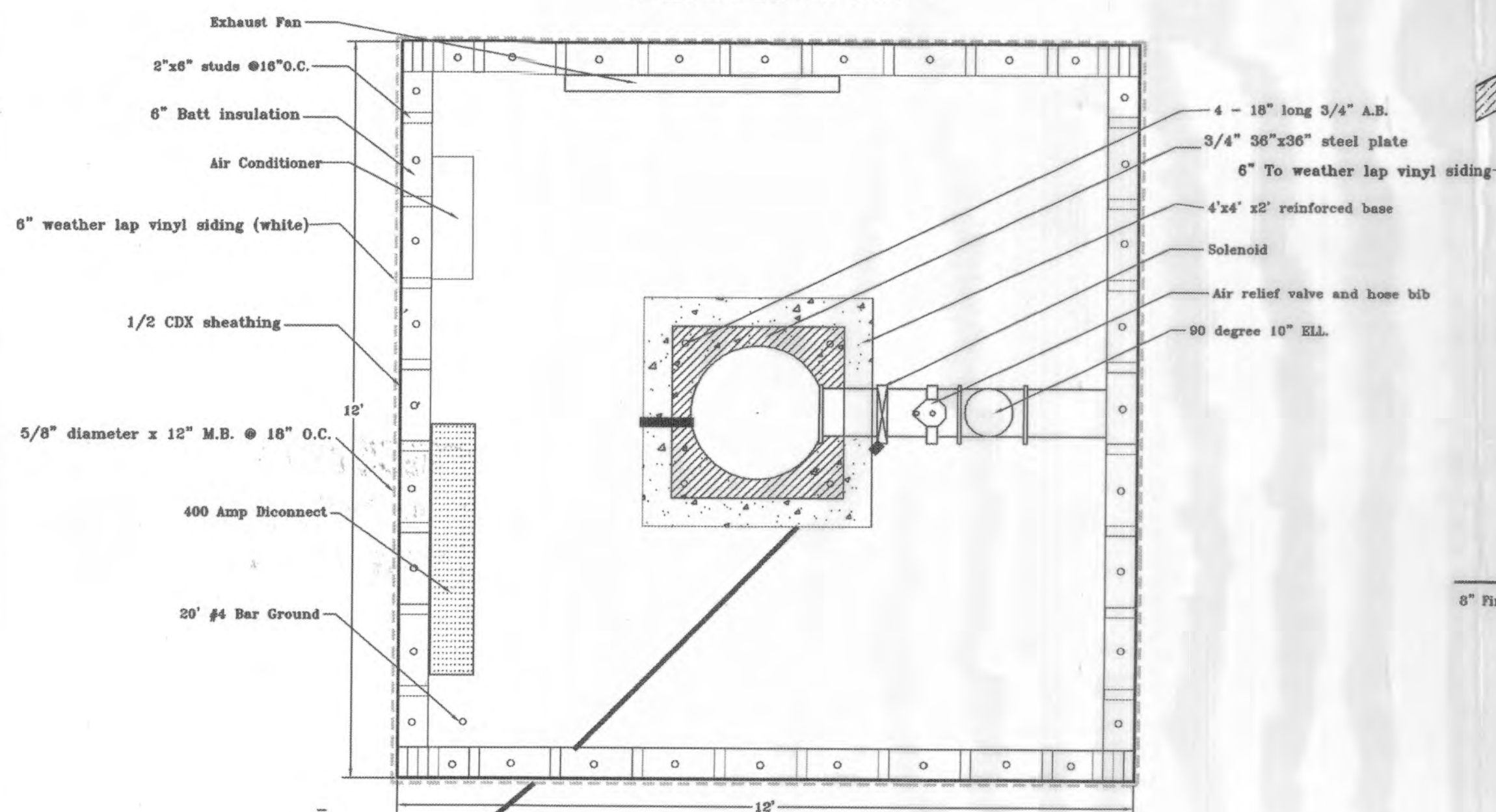
PLAN
