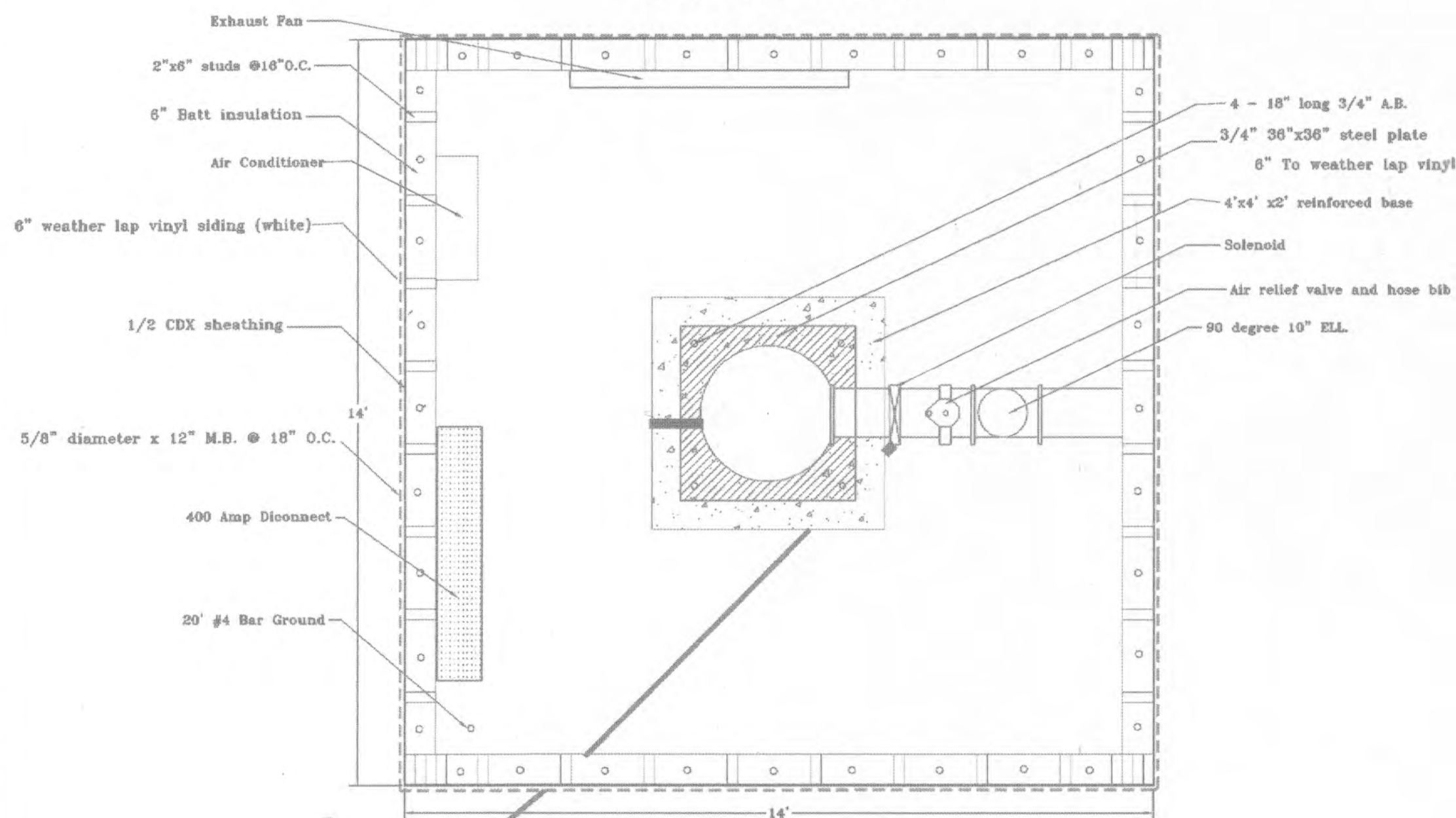
PLAN
