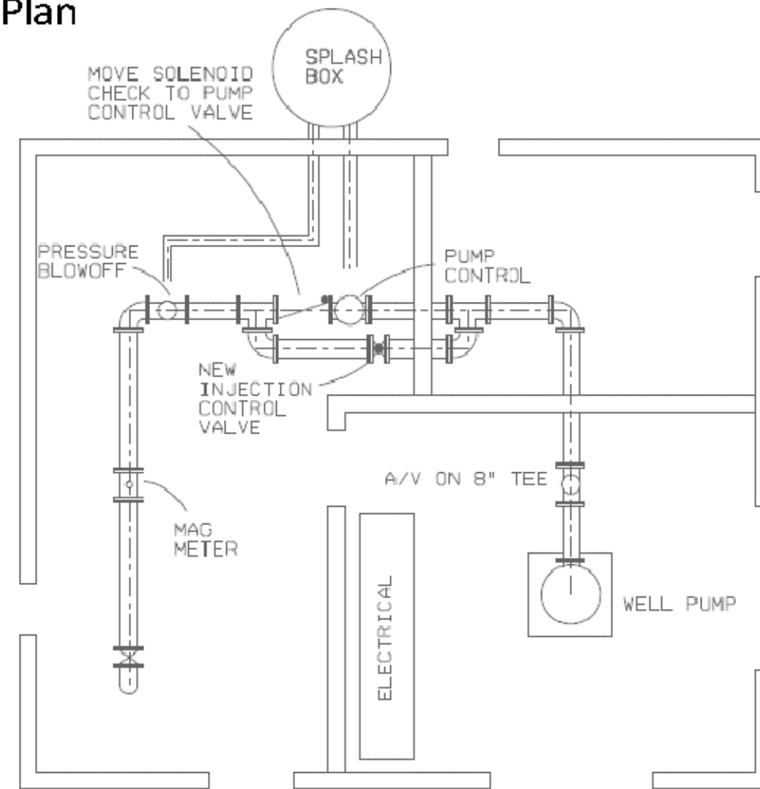
MODIFIED PIPING
