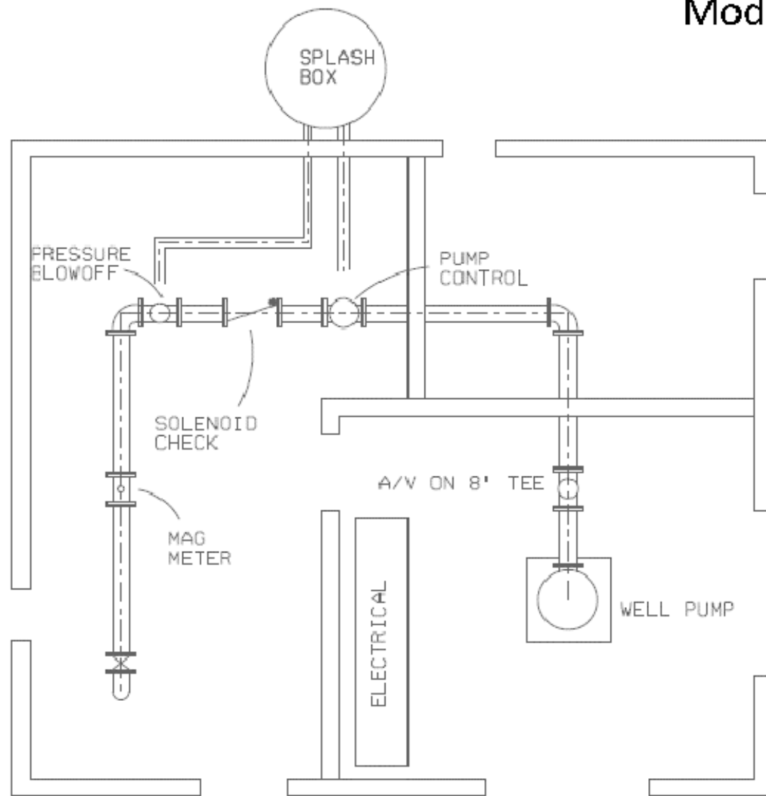
EXISTING PIPING
