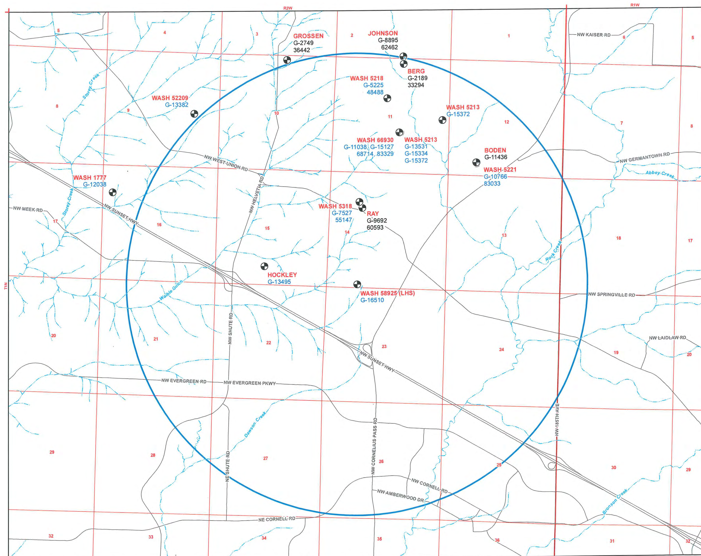
Allocation of Groundwater in Area Affected by ASR Hillsboro School District Liberty High School ASR Evaluation
