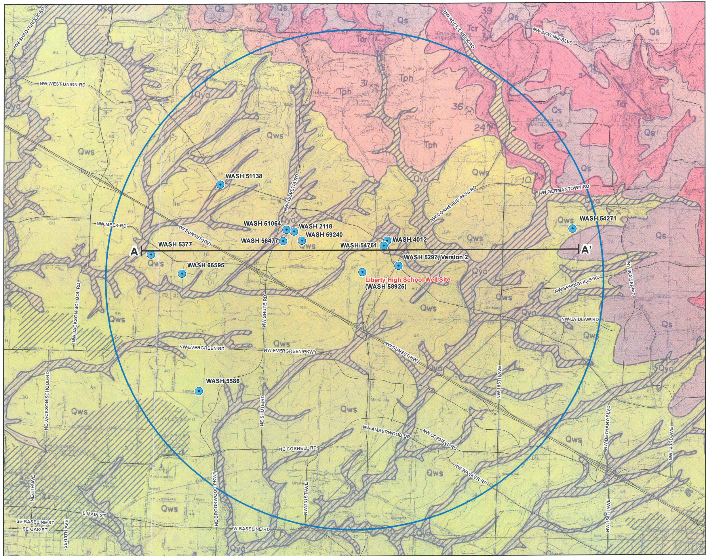
FIGURE 4 Geologic Map Hillsboro School District Liberty High School ASR Evaluation
