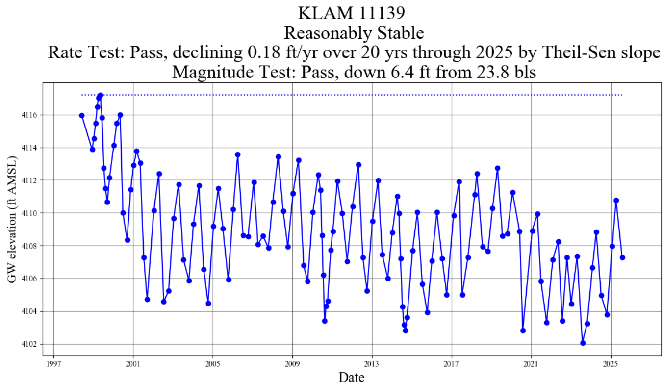
Figure 5 – Hydrograph for KLAM 11139
