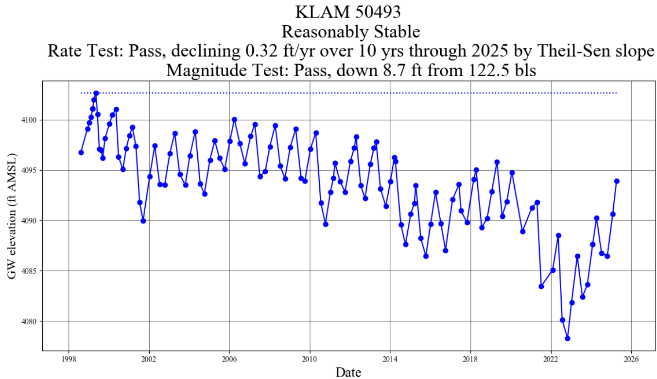
Figure 7 – Hydrograph for KLAM 50493
