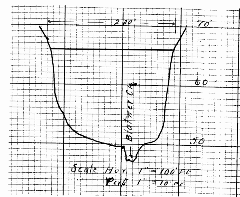
SECTION AT DAM.
