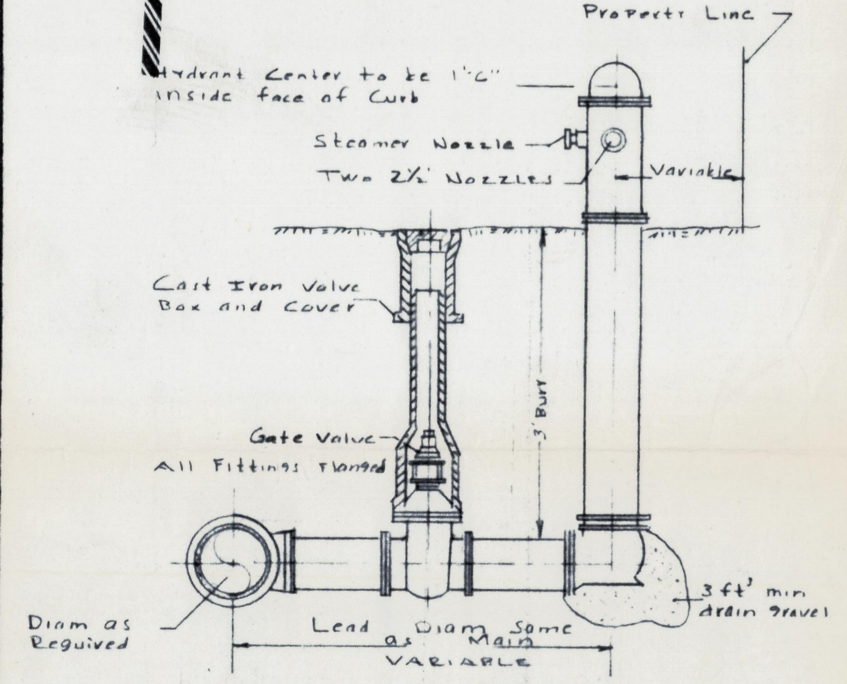
TYPICAL HYDRANT ASSEMBLY OPTIONAL AS REQ'D BY WATER DIST.
