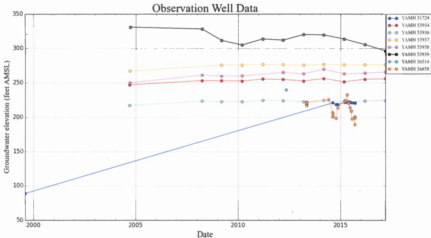
Figure 3. There are no wells with long-term water level data located within a mile of the subject well. Water level data from marine sedimentary rock wells located more than two miles to the southeast are the nearest data available, and they show reasonably stable trends under the current level of use.
