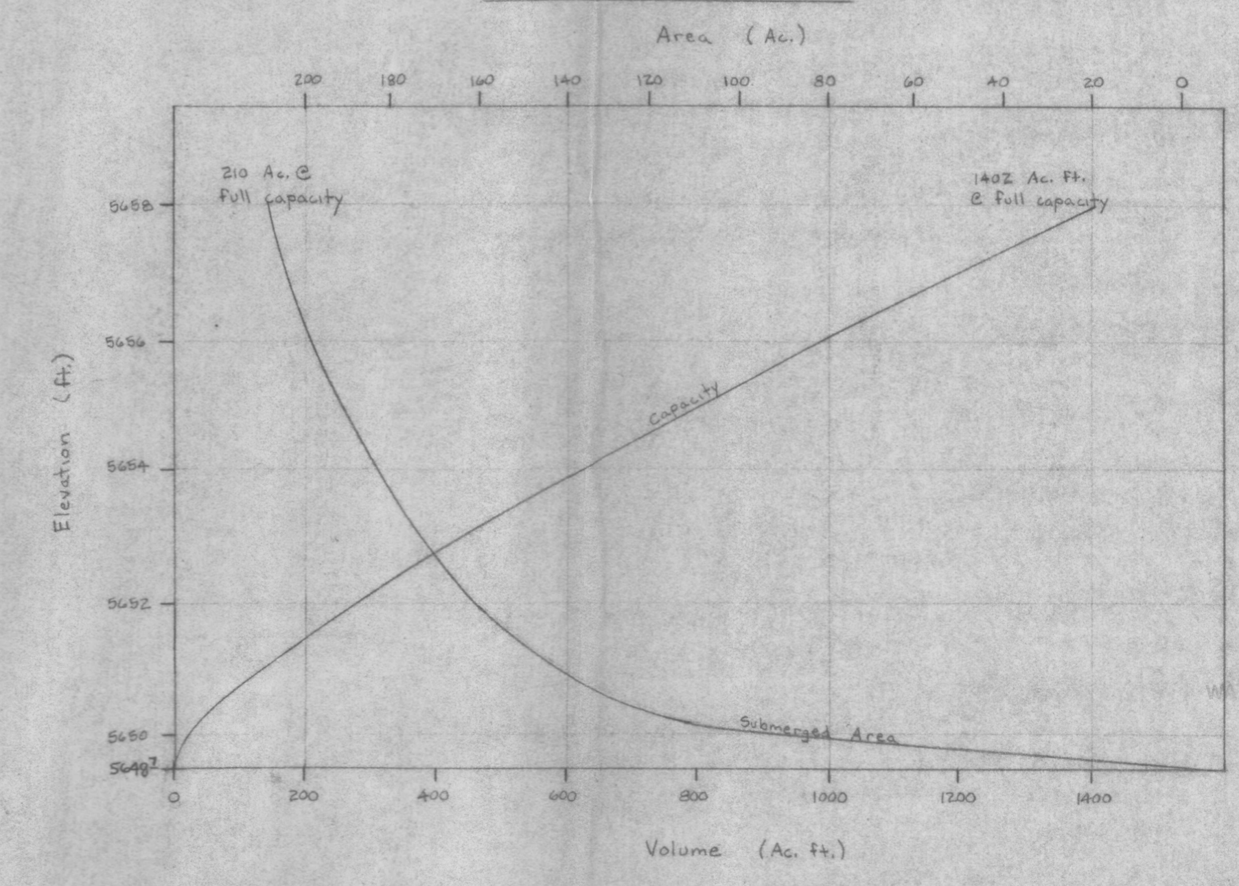
Capacity - Area Curves
