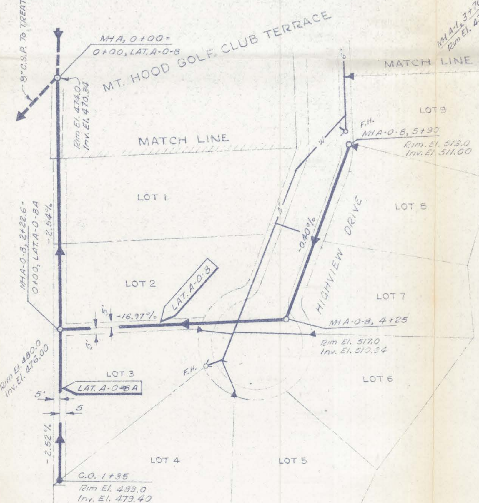
INSET MT. HOOD GOLF CLUB TERRACE NO. 2
