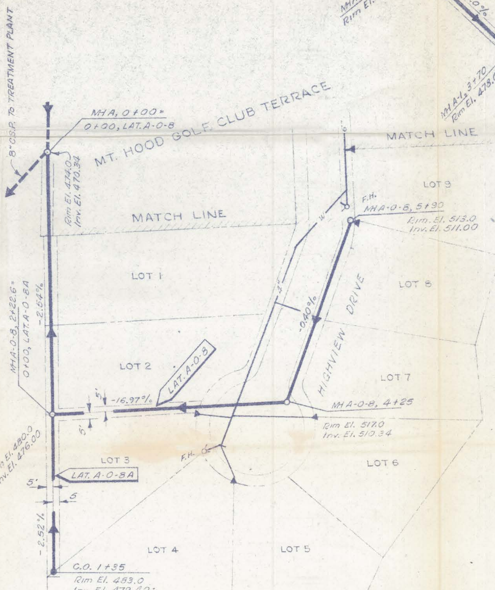
INSET MT. HOOD GOLF CLUB TERRACE NO. 2
