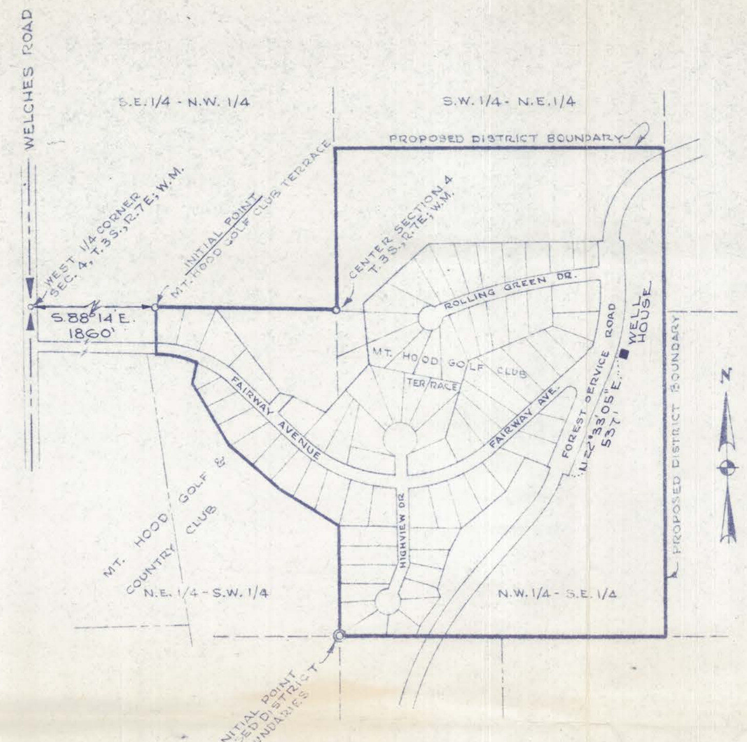
PROPOSED DISTRICT BOUNDARIES MT. HOOD GOLF SANITARY DISTRICT GOLF CLUB TERRACE WATER DISTRICT SCALE: 1" = 400'
