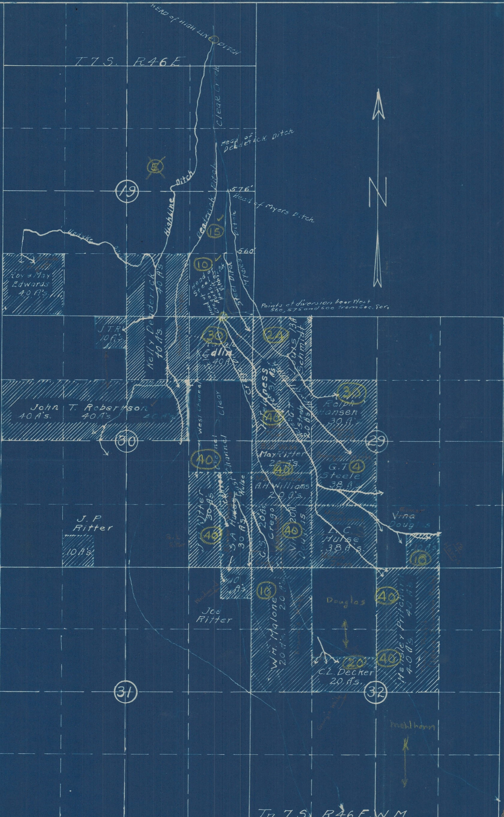
Map to accompany proof of Appropriation of Water Permit No. R-515 Clear Creek Reservoir Company Halfway, Baker County, Oregon Scale 1"=1200' Map drawn by H.T. Swan, Baker Oregon
